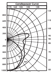
KC2300 White 4' Reflector with Perforated Basket
