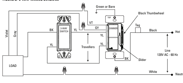
FIGURE 2: 3-WAY WIRING DIAGRAM
