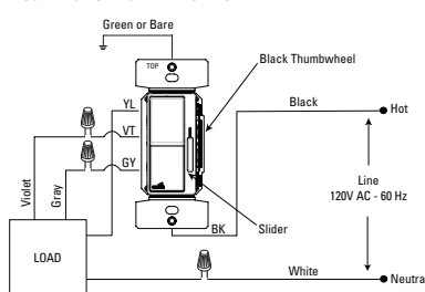
FIGURE 1: SINGLE POLE WIRING DIAGRAM
