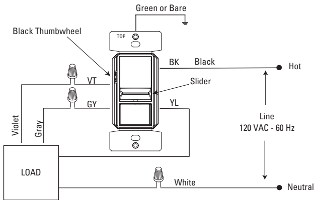
FIGURE 1: SINGLE-POLE WIRING DIAGRAM
