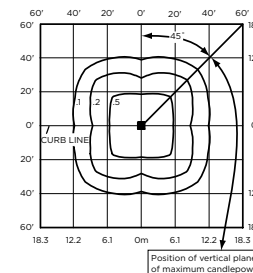
VG-A-**-5W-A-40K-UL Mounting Height: 10' (3.0m) A.F.G. Initial Delivered Lumens: 3,760 Initial FC at grade
