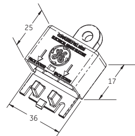
Weather Box
