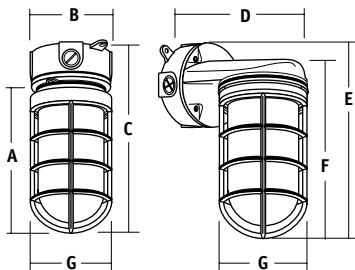
150 Watt Lugs: 5" center to center
