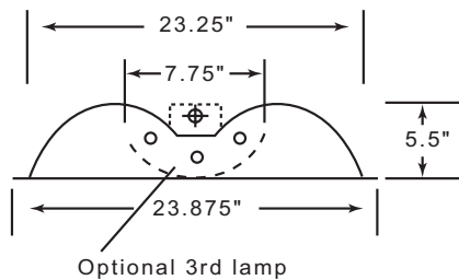
END VIEW T5
