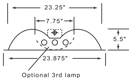
END VIEW T8
