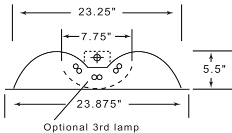
END VIEW Biax
