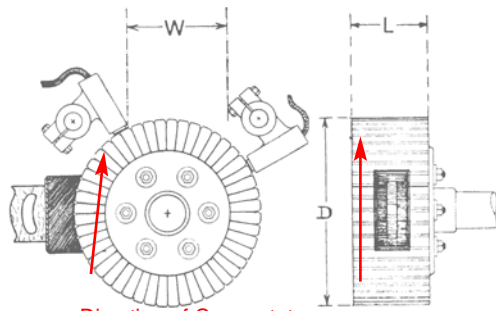
Direction of Commutator Rotation, as shown by arrow.
