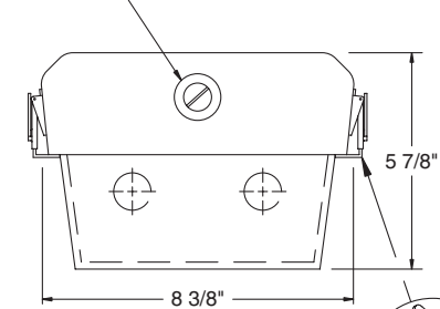
1/2" THREADED HUB (WIRE ENTRY)
