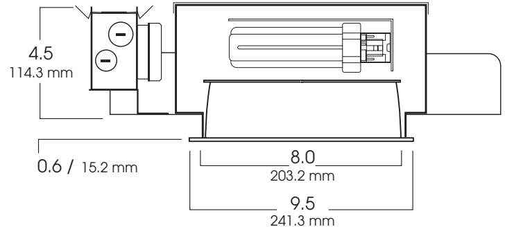
CROSS-SECTION
