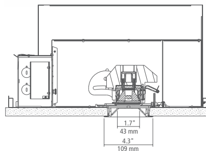
IC AIRTIGHT, SHOWN AS FLANGED
