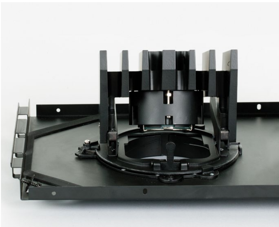
-Aluminum heat sink designed for precise LED aiming to maximize output and for superior heat dissipation
