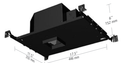
IC AIRTIGHT, SHOWN AS FLANGED
