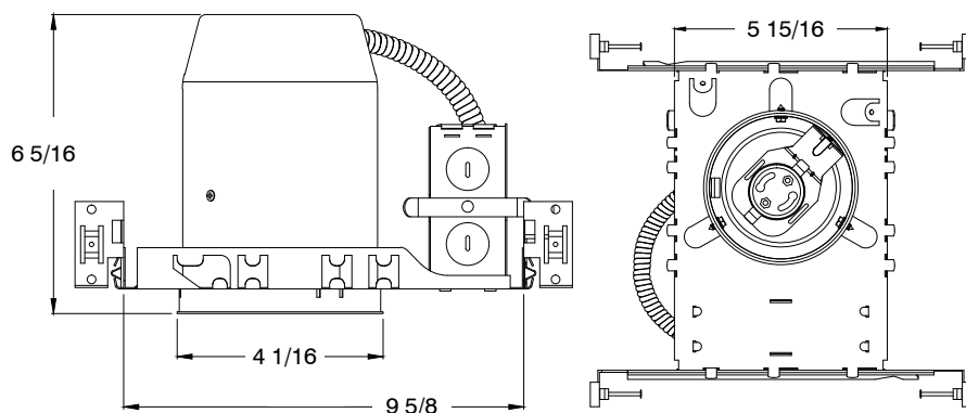
GU24 Socket
