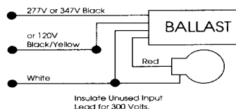
Wiring Diagram 34
