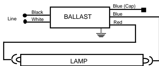
ONE LAMP APPLICATION Cap any blue lead, insulate to 600 volts
