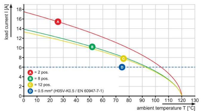
BCL-SMT 3.81/./90 - SCZ 3.81/./180
